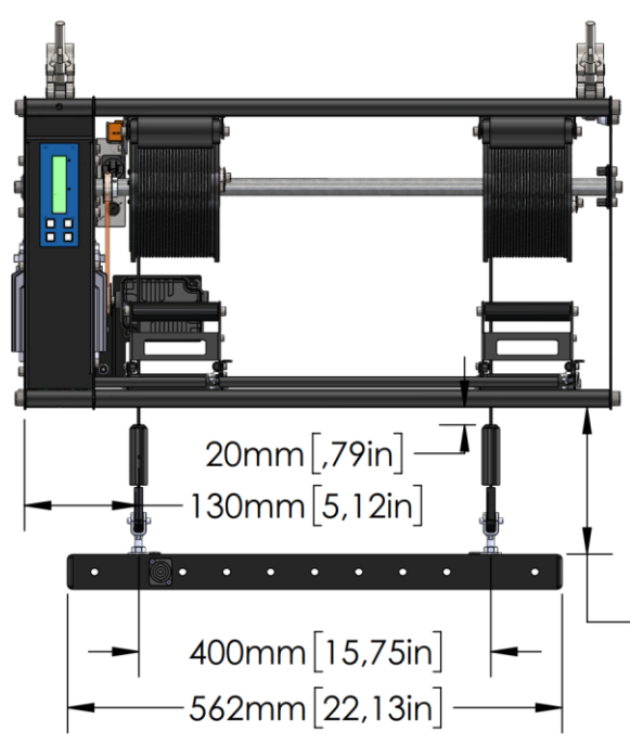
FRONT VIEW TOP POSITION
