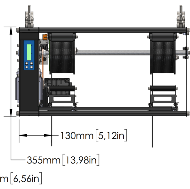
FRONT VIEW BOTTOM POSITION
