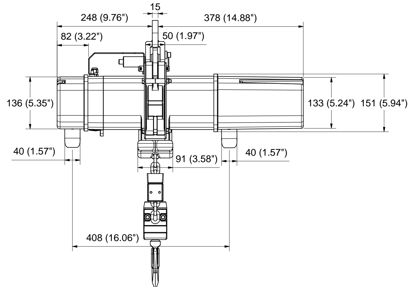
SIDE VIEW
