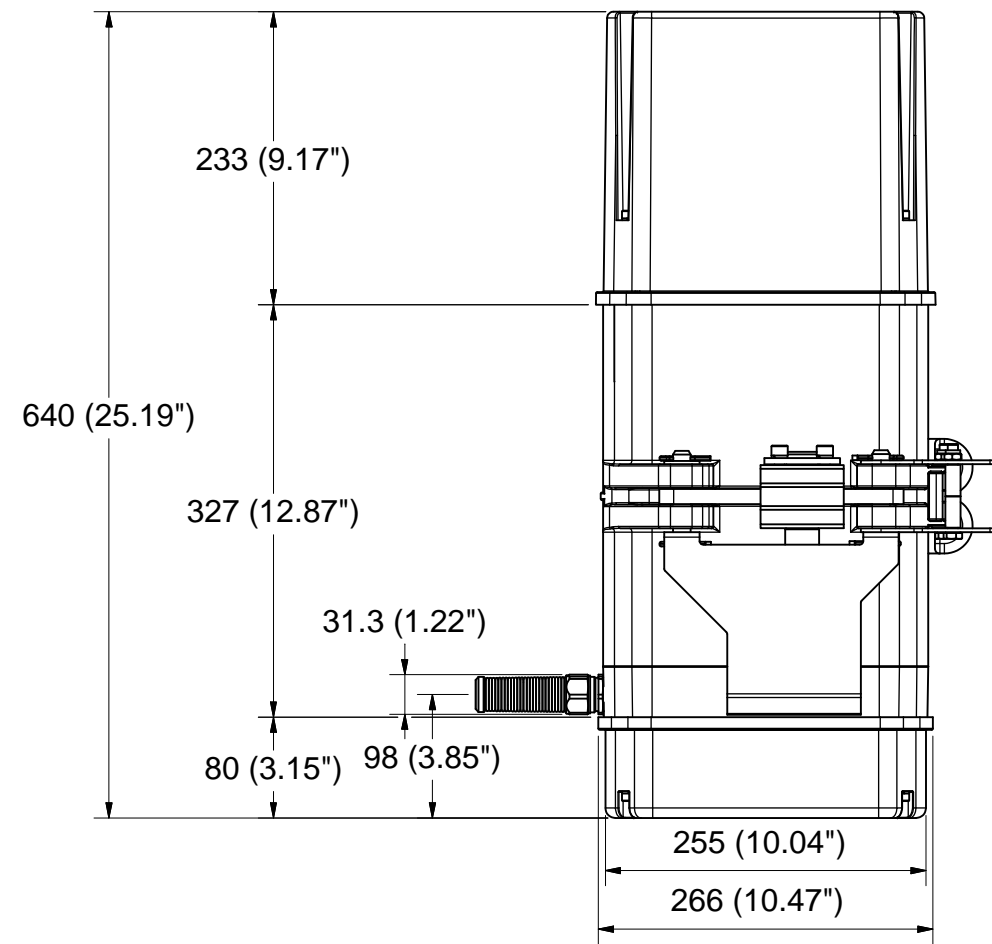
TOP VIEW
